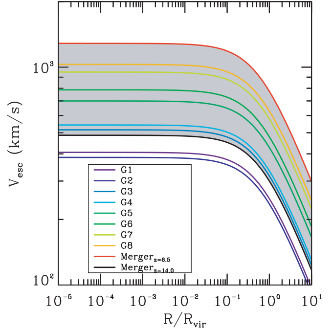
FIG. 4.— Halo escape velocity V_{\text{esc}} as a function of distance R/R_{\text{vir}} ( R_{\text{vir}} is the virial radius) to the halo center for various models in our merger simulations. This plot includes the isolated halo progenitors G1–G8 in Table 1, as well as the first merger remnant at z \simeq 14 and the last one at z \simeq 6.5 , as labeled in the legend. The shaded region indicates the range of the escape velocities of the mergers in our simulations, with the values in the central regions being 486 \text{ km s}^{-1} \lesssim V_{\text{esc}} \lesssim 1284 \text{ km s}^{-1} .
