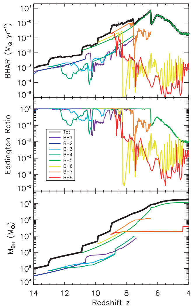
FIG. 10.—Growth history of the quasar system, including the BH accretion rate BHAR ( top ), the Eddington ratio L_{\text{bol}}/L_{\text{Edd}} ( middle ), and BH mass ( bottom ). Note that the black lines represent totals, while colored lines show individual BHs, as indicated in the legend.
