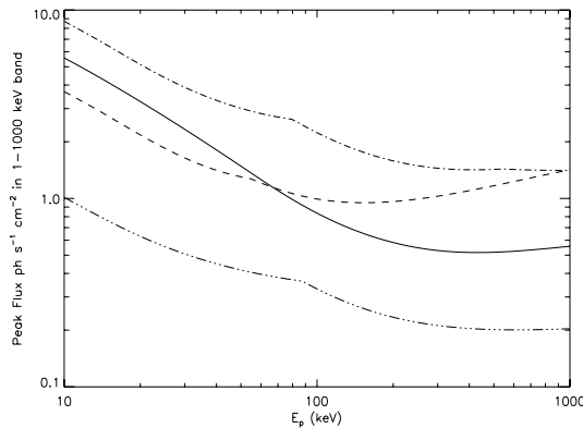
FIGURE 1. Threshold value of F_T (1–1000 keV peak flux) as a function of E_p for BATSE (solid), the BAT (dashed), the GBM (dot-dashed) and one EXIST telescope (3 dots-dashed). The spectrum has a low energy spectral index of \alpha = -0.5 and a high energy index of \beta = -2 .
