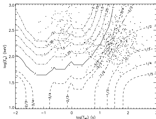
FIGURE 3. Contour plot of the ratio of the sensitivities of the BAT and BATSE as a function of E_p and T_{90} ; a ratio less than one indicates that the BAT is more sensitive than BATSE. \alpha=-0.5 and \beta=-2 are assumed. Also plotted are the E_p and T_{90} for a set of BATSE bursts with enough counts for spectral fits.
