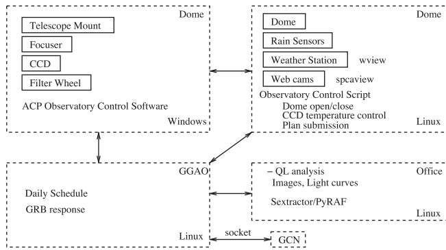
Fig. 6. Flowchart of GRT automation.
