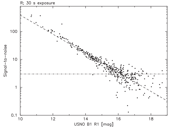
Fig. 7. Relationship between signal-to-noise ratio and the R1 magnitude of the USNO B1 catalog for the image of the field of GRB 100915 at a 30 s exposure in the R filter. The horizontal dash-dotted line shows the 3\sigma detection limit.
