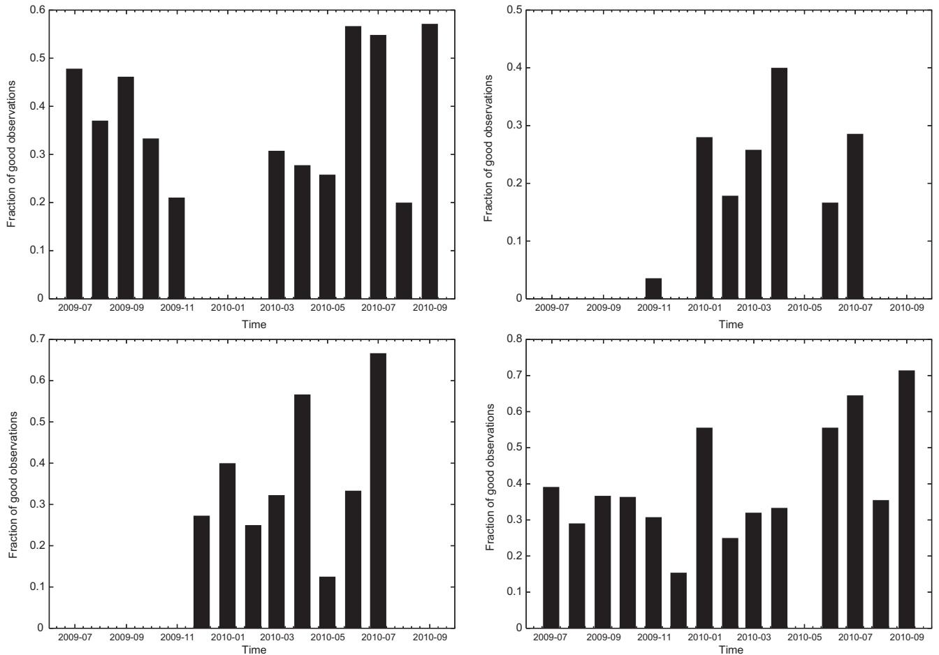
Fig. 9. Fraction of good observations for each month for four AGN observations: Mrk 501 (top left), Mrk 421 (top right), 3C273 (bottom left) and IES 1959+650 (bottom right).
