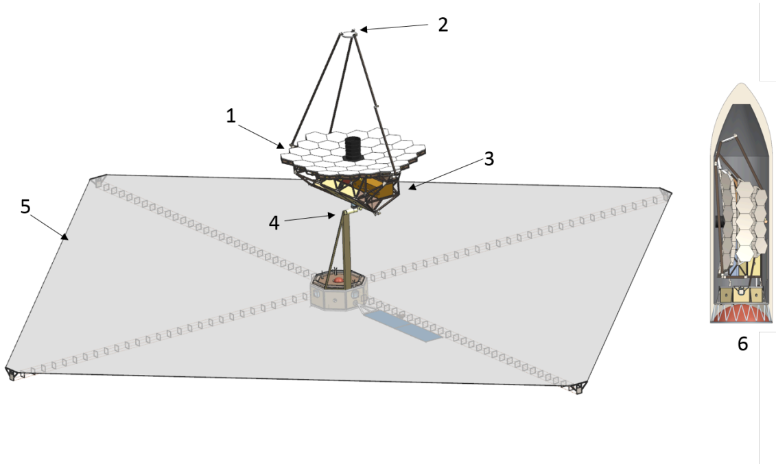
Figure 1 – The ATLAST reference architecture. The primary mirror (1) consists of 36 JWST-sized segments made from either glass or SiC that would use segment heater plates to maintain thermal stability. The secondary mirror (2) is actively controlled in six degrees-of-freedom using metrology referenced to the science instrument module. The science instruments (3) are externally accessible for serviceability. The entire telescope is isolated from the spacecraft via a non-contact pointing gimbal system (4). The gimbal mount allows full access to the field-of-regard while maintaining a constant view-angle between the three layer sunshield (5) and the sun, providing a stable thermal sink. Using multiple chord-folds similar to those used on JWST, the entire system can be stowed (6) inside of a typical 5-m fairing.
