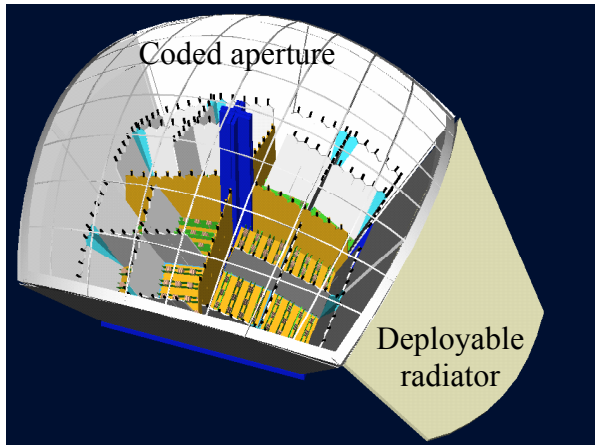
FIGURE 7. Partial detail of concept EXIST-ISS telescope (1 of 2; cf. Fig. 1) showing CZT arrays ( 16 \times 2500\text{cm}^2 ), CsI collimators, and extended coded aperture mask and supporting structures.
