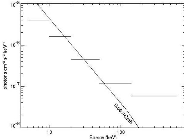
FIGURE 2. Approximate continuum sensitivity ( 5\sigma , 1 year) for EXIST-ISS configuration. Narrow line sensitivities ( \text{phot}/\text{cm}^2\text{-sec} ) are reduced by factor of \sim 10 .
