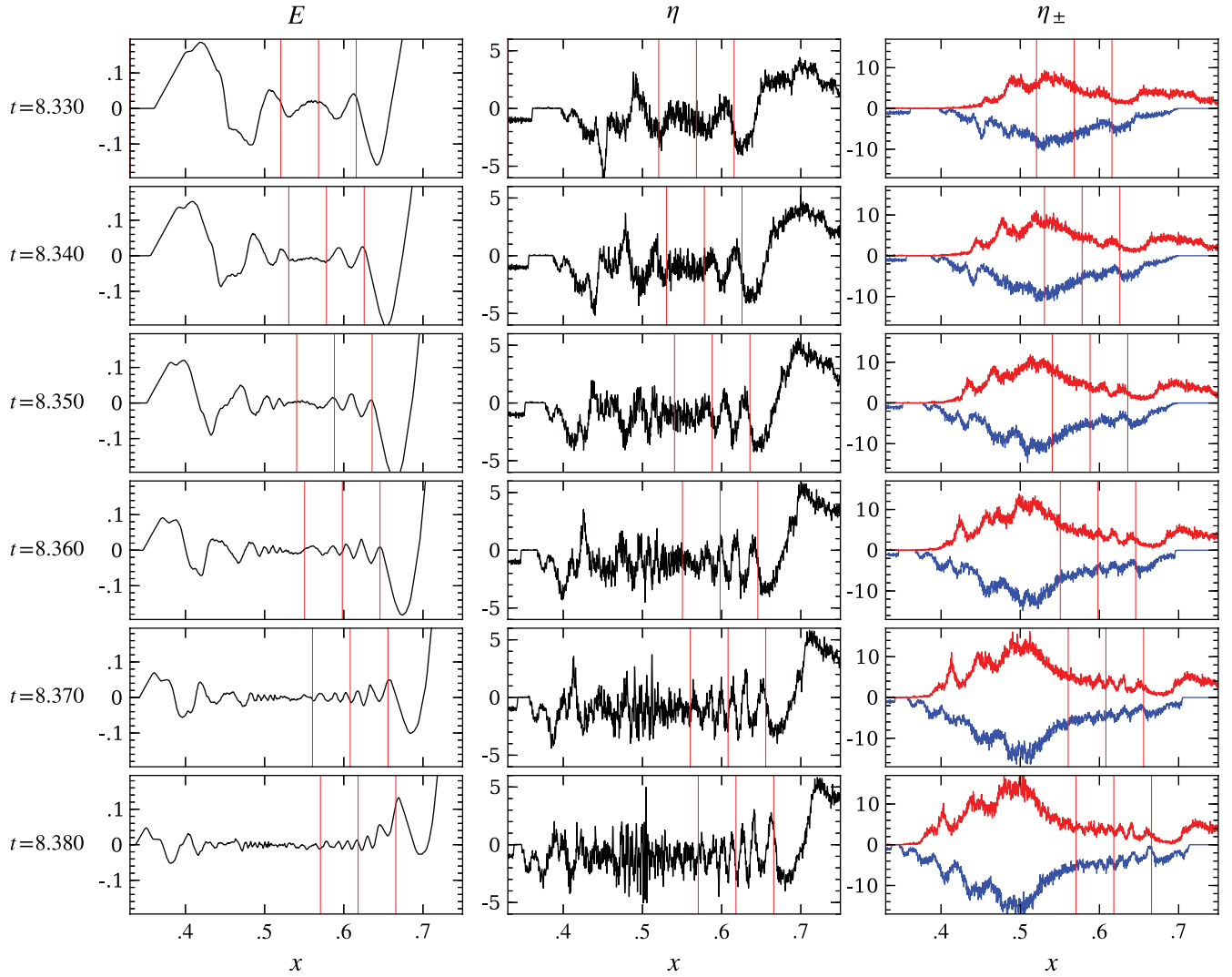
Figure 19. Screening of the electric field and formation of superluminal electrostatic wave for cascade with j_m = -0.5j_{GJ} . There are six snapshots for the electric field E , the total charge density \eta and the charge density of electrons (negative values, blue line) and positrons (positive values, red line) \eta_{\pm} . All quantities are plotted as functions of distance x for the part of the calculation domain with intense pair formation. Snapshots are taken at equally separated time intervals. Plots in each column are aligned and share the same values of x . The same normalizations for physical quantities are used as in Fig. 11. The three thin red vertical lines in each plot mark fiducial points moving with the speed of light towards the magnetosphere.
