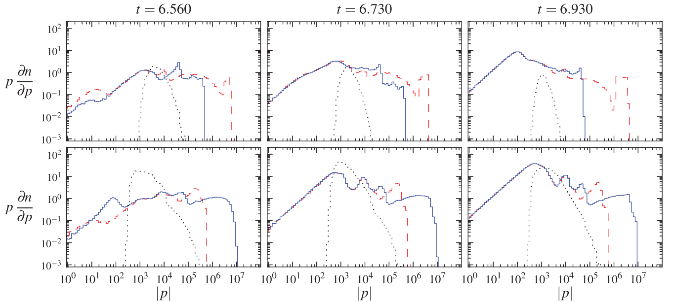
Figure 18. Momentum distributions of particles at three moments of time for cascade with anti-GJ current density j_m = -1.5j_{GJ} . Notations are the same as in Fig. 17. The following spacial regions were used for plotting the average distribution functions: x \in [0, 0.75] for t = 6.560 , x \in [0, 0.88] for t = 6.730 and x \in [0, 1] for t = 6.930 .
