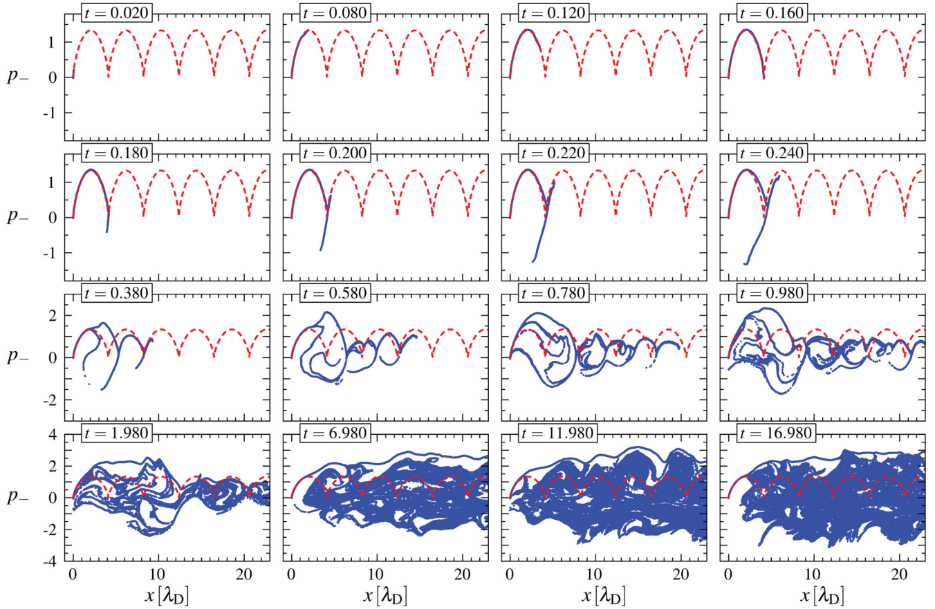
Figure 5. Development of ‘trapped particle’ flow when the space charge limited flow which starts into vacuum. Phase space portrait of particles are shown for 16 moments of time indicated in small boxes on the top of each plot. The current density j_m = 0.5j_{GJ} . The distance x is measured in units of the Debye length. Red dashed lines show the analytical solution for stationary flow. Particle momenta p_- are normalized to m_e c . The total length of the computational domain L = 50\lambda_{D,GJ} , only part of it ( x < 50\lambda_{D,GJ} ) is shown here. Time is measured in fly-by time ( L/c ) of the whole domain. Snapshots in the same row have the same time interval between them, but these time intervals are different for different rows; they increase towards the bottom row.
