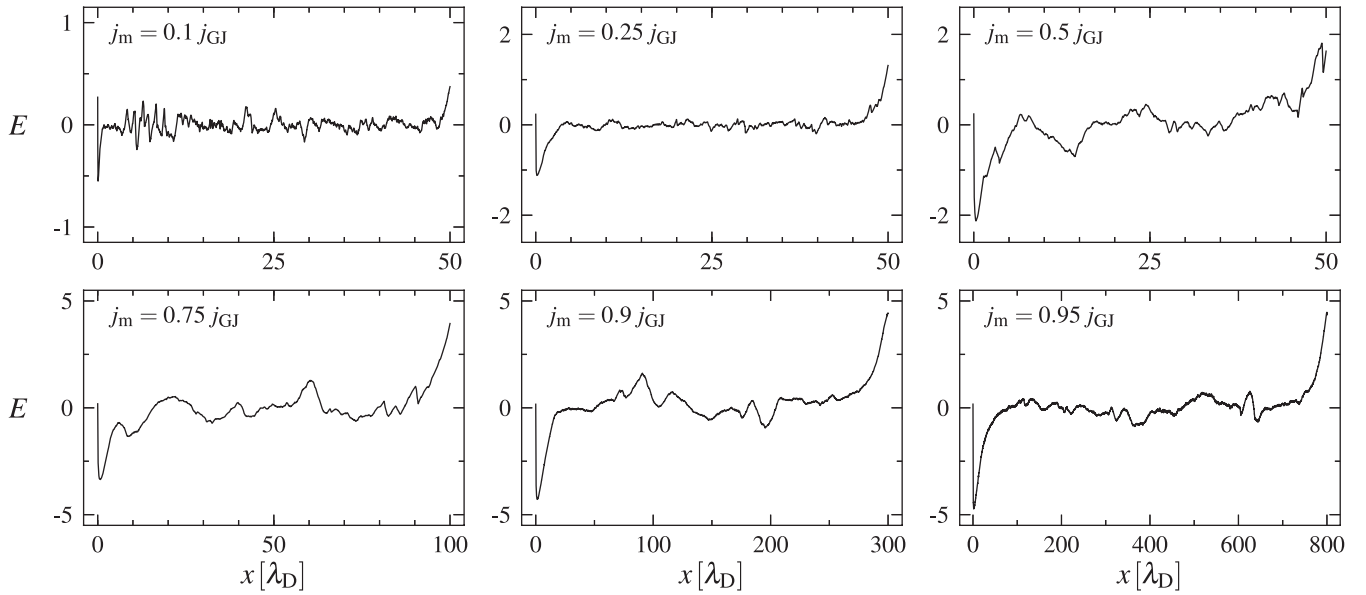
Figure 8. Snapshots of the electric field E for well-developed space charge limited flows taken at the same moment as the phase space portraits from Fig. 6. E is normalized to \pi \eta_{\text{GJ}} \lambda_{\text{D}} j_{\text{GJ}} .
