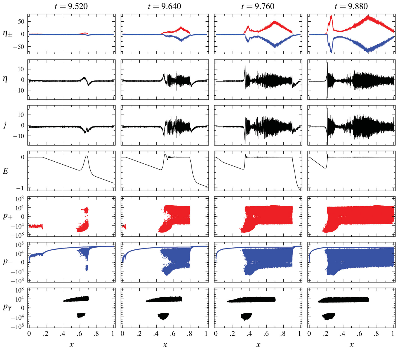
Figure 21. Screening of the electric field in super-GJ flow with j_m = 1.5j_{GJ} . The same quantities are plotted as in Fig. 11.
