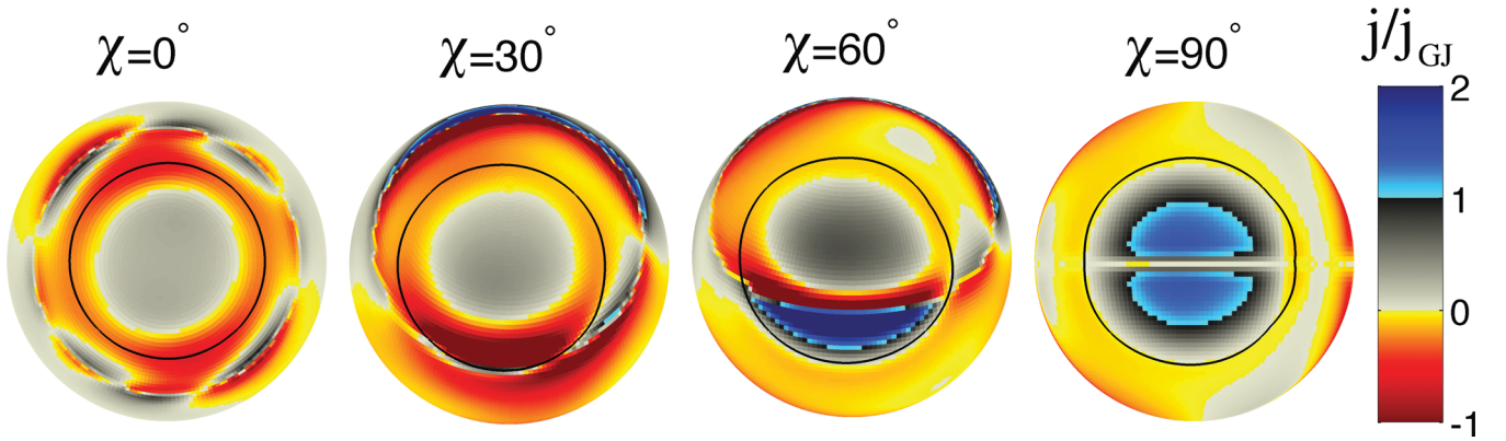
Figure 1. Field-aligned current density at the polar cap of the force-free rotator, with j_{\parallel} measured in units of the Goldreich–Julian current density j_{\text{GJ}} \equiv -\boldsymbol{\Omega} \cdot \boldsymbol{B}/2\pi c . The black circle is the rim of the polar cap – the footprints of the field lines that pass outside the light cylinder fall with that circle. The distributed current is shown. The current sheet component coincides with the polar cap boundary. This plot was made by Xuening Bai using results of force-free magnetosphere simulations presented in Bai & Spitkovsky (2010).
