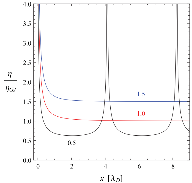
Figure 4. Charge density of stationary space charge limited flow normalized to the GJ charge density \eta_{GJ} as a function of distance x normalized to \lambda_D for current densities j_m/j_{GJ} = 0.5, 1.0, 1.5 .
