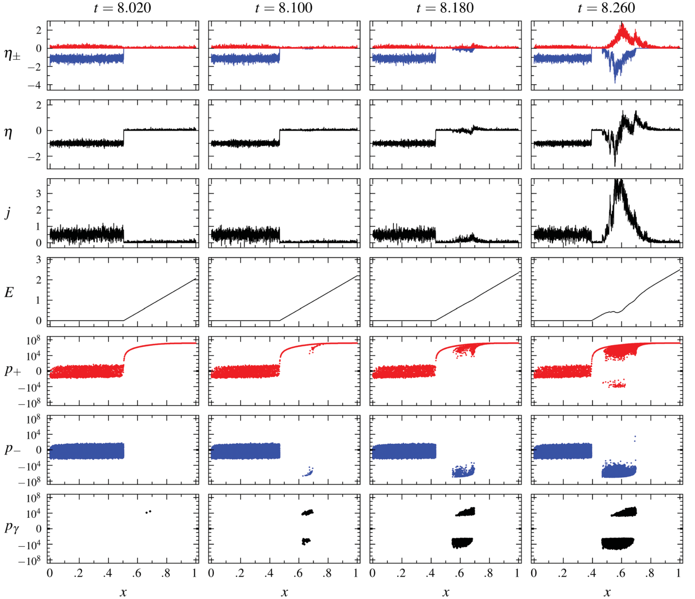
Figure 11. Ignition of pair formation in anti-GJ flow with j_m = -0.5j_{\text{GJ}} . Several physical quantities are shown as functions of the distance x from the NS; x is normalized to the domain size L . Plots in each column (for the same time t ) are aligned – they share the same values of x . The following quantities are plotted: first row: \eta_{\pm} – charge density of electrons (negative values, blue line) and positrons (positive values, red line); \eta_{\pm} is normalized to the absolute value of the Goldreich–Julian charge density |\eta_{\text{GJ}}| . Second row: the total charge density \eta normalized to the absolute value of the Goldreich–Julian charge density |\eta_{\text{GJ}}| . Third row: current density j normalized to the absolute value of the Goldreich–Julian current density |j_{\text{GJ}}| \equiv |\eta_{\text{GJ}}c| . Fourth row: accelerating electric field E normalized to the ‘vacuum’ electric field E_0 \equiv |\eta_{\text{GJ}}|rL . Fifth row: phase space portrait of positrons (horizontal axis – positron position x , vertical axis – positron momentum p_+ normalized to m_e c ). The vertical axis is logarithmic except for the region around zero momentum ( -5 < p_+ < 5 ), where the scale is linear. Sixth row: phase space portrait of electrons (horizontal axis – electron position x , vertical axis – electron momentum p_- normalized to m_e c ). Seventh row: phase space portrait of pair-producing photons (horizontal axis – photon position x , vertical axis – photon momentum p_\gamma normalized to m_e c ).
